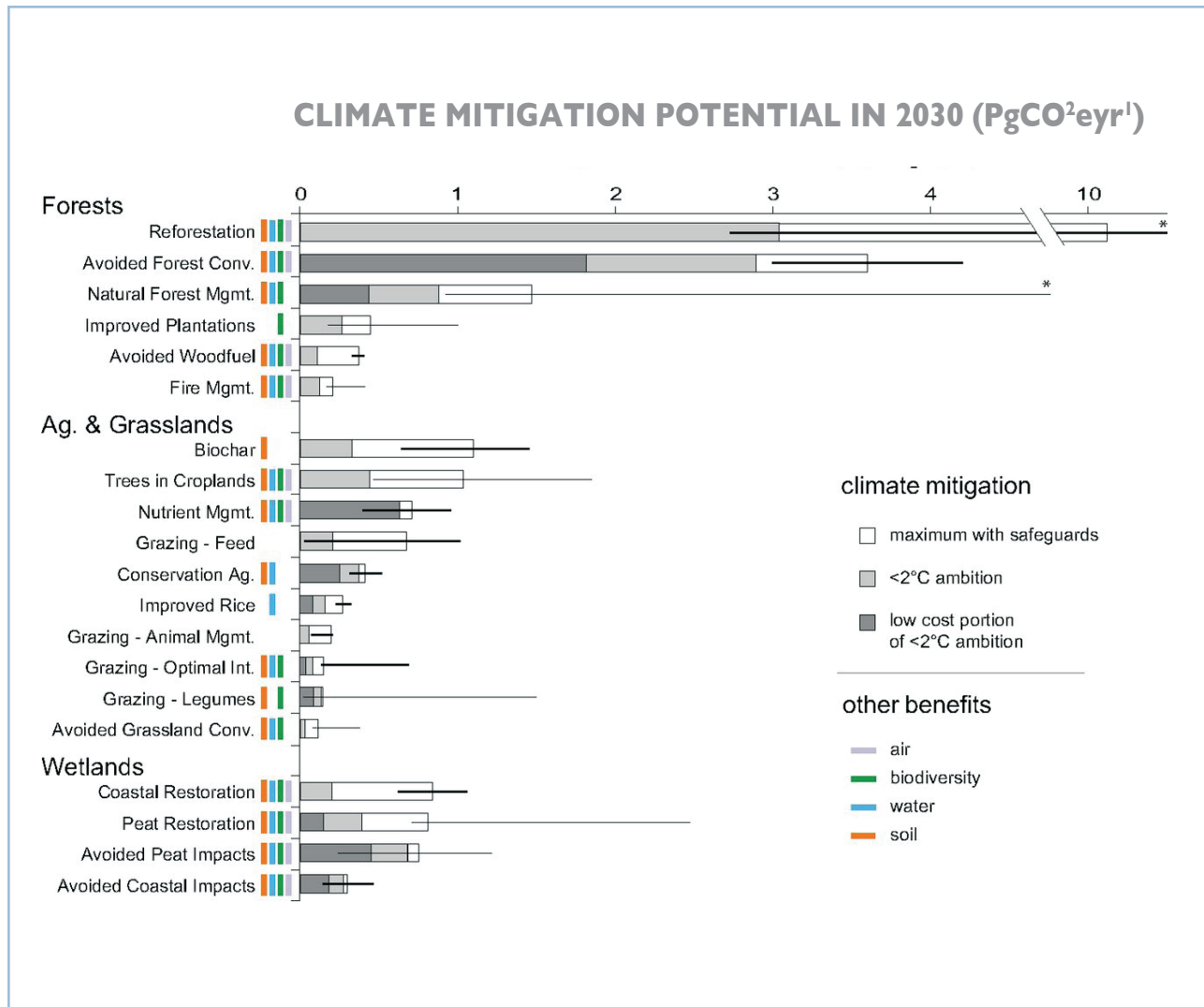
FIGURE 2. The maximum additional mitigation potential for natural pathways in the year 2030 considering differing degrees of climate mitigation (illustrated with gray shading). Ecosystem service benefits (listed as “other benefits”) linked with each pathway are indicated by colored bars listed with each category on the left side of the figure.
